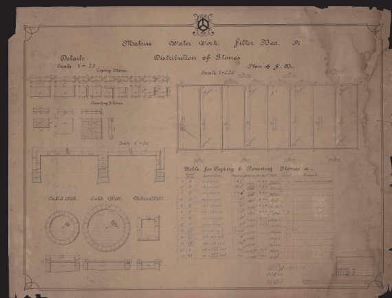
2. Matsue Water Work Filter Bed (表面)
